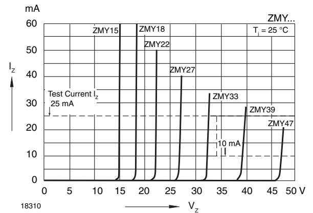
Fig. 5 - Typical Breakdown Characteristics
