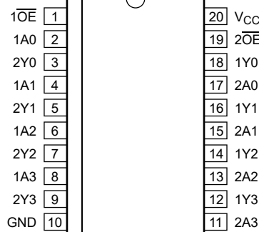
D package SOT163-1 (SO20)
