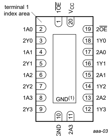
BQ package SOT764-1 (DHVQFN20)
