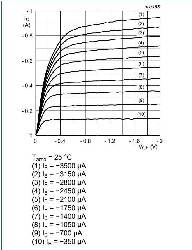
Fig. 5. Collector current as a function of collector-emitter voltage; typical values
