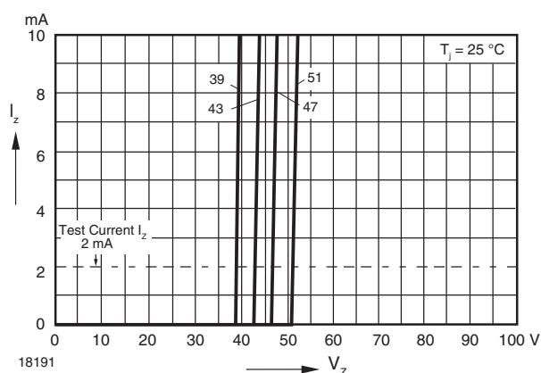
Fig. 16 - Breakdown Characteristics
