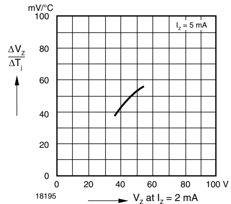
Fig. 11 - Temperature Dependence of Zener Voltage vs. Zener Voltage
