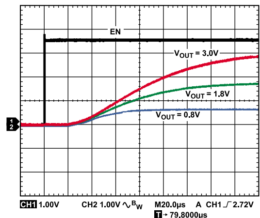
Figure 29. Typical Start-Up Time
