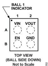
Figure 2. Pin Configuration
