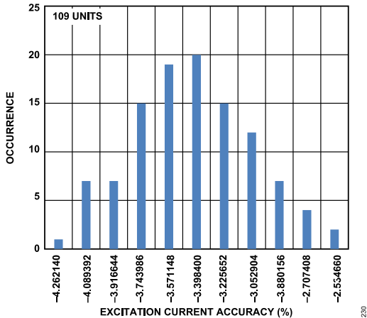
Figure 31. IOUTx Current Initial Accuracy Histogram (500 \mu A)
