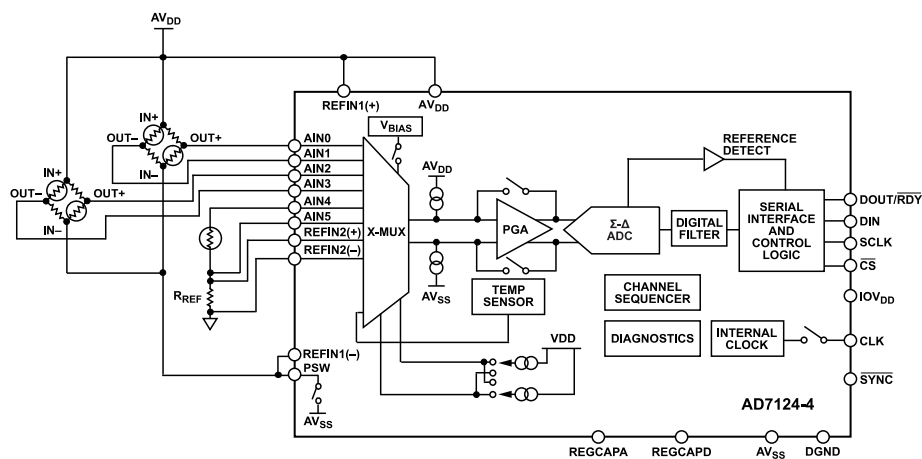
Figure 129. Flowmeter Application
