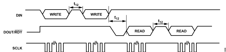
Figure 6. Delay Between Consecutive Serial Operations
