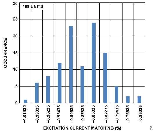
Figure 32. IOUTx Current Initial Matching Histogram (500 \mu A)
