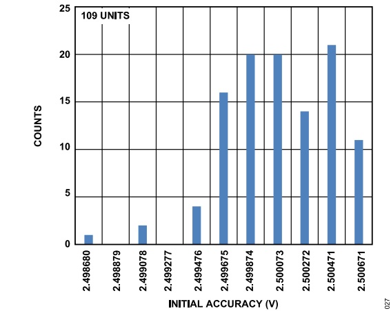
Figure 29. Internal Reference Voltage Histogram
