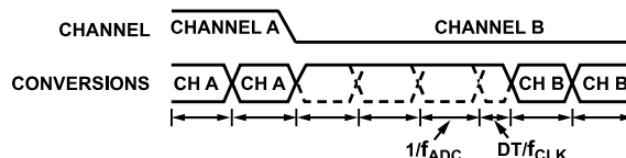
Figure 91. Sinc³ Channel Change
