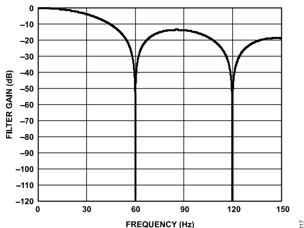
Figure 108. 60 Hz Rejection
