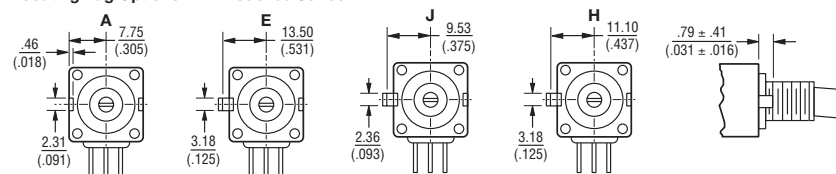
Locating Lug Options - All Model 80 Series
