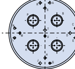
ARRANGEMENT 19Q-18 14X SIZE 22D 4X SIZE 8 QUADRA
