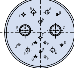
ARRANGEMENT 19Q-17 10X SIZE 22D 1X SIZE 20 4X SIZE 16 2X SIZE 8 QUADRA
