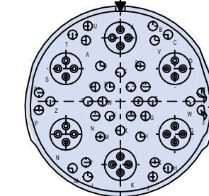
ARRANGEMENT 25Q-17 36X SIZE 22 6X SIZE 8 QUADRA
