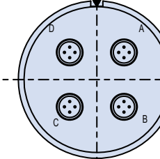
ARRANGEMENT 21Q-75 4X SIZE 8 QUADRA
