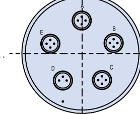
ARRANGEMENT 23Q-05 (IAW PREN 3645-001) 5X SIZE 8 QUADRA
