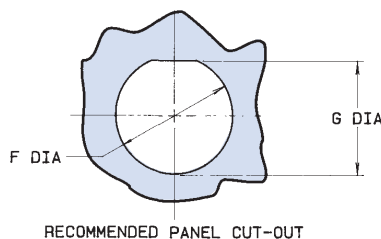
SHELL SIZE A THREAD CLASS 2A B DIA MAX C MAX D HEX E FLATS F DIA .005(0.1) G +.000-.005 (0-0.1) 09 .688-24 UNEF .573(14.6) .900(22.9) .875(22.2) 1.062(27.0) .703(17.9) .699(17.8) 11 0.813-20 UNEF .701(17.8) 1.030(26.2) 1.000(25.4) 1.250(31.8) .827(21.0) .769(19.5) 13 1.000-20 UNEF .851(21.6) 1.205(30.6) 1.188(30.2) 1.375(34.9) 1.015(25.8) .955(24.3) 15 1.125-18 UNEF .976(24.8) 1.325(33.7) 1.312(33.3) 1.500(38.1) 1.140(29.0) 1.084(27.5) 17 1.250-18 UNEF 1.101(28.0) 1.450(36.8) 1.438(36.5) 1.625(41.3) 1.265(32.1) 1.208(30.7) 19 1.375-18 UNEF 1.208(30.7) 1.565(39.8) 1.562(39.7) 1.812(46.0) 1.390(35.3) 1.333(33.9) 21 1.500-18 UNEF 1.333(33.9) 1.690(42.9) 1.688(42.9) 1.938(49.2) 1.515(38.5) 1.459(37.1) 23 1.625-18 UNEF 1.458(37.0) 1.795(45.6) 1.812(46.0) 2.062(52.4) 1.640(41.7) 1.580(40.1) 25 1.750-18 UNS 1.583(40.2) 1.920(48.8) 2.000(50.8) 2.188(55.6) 1.765(44.8) 1.709(43.4)
