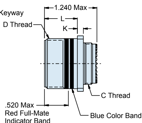
S7 - WALL MOUNT RECEPTACLE
