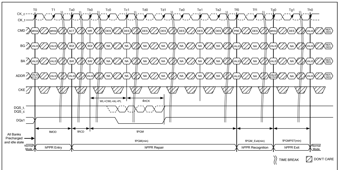
Figure 159 – Hard Fail Row Repair (WR Case)
