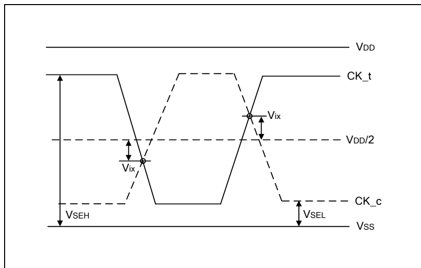
Figure 184 – Vix Definition (CK)
