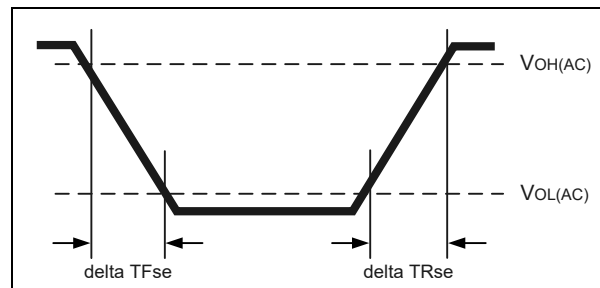
Figure 191 – Single-ended Output Slew Rate Definition
