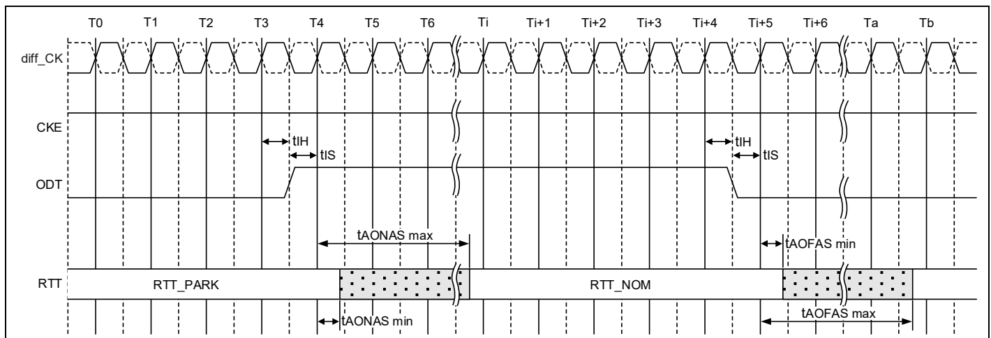
Figure 169 – Asynchronous ODT Timing on DDR4 SDRAM with DLL-off ODT Timing on DDR4 SDRAM with DLL-off
