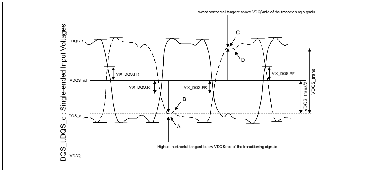
Figure 188 – Vix Definition (DQS)
