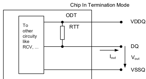
Figure 162 – On Die Termination
