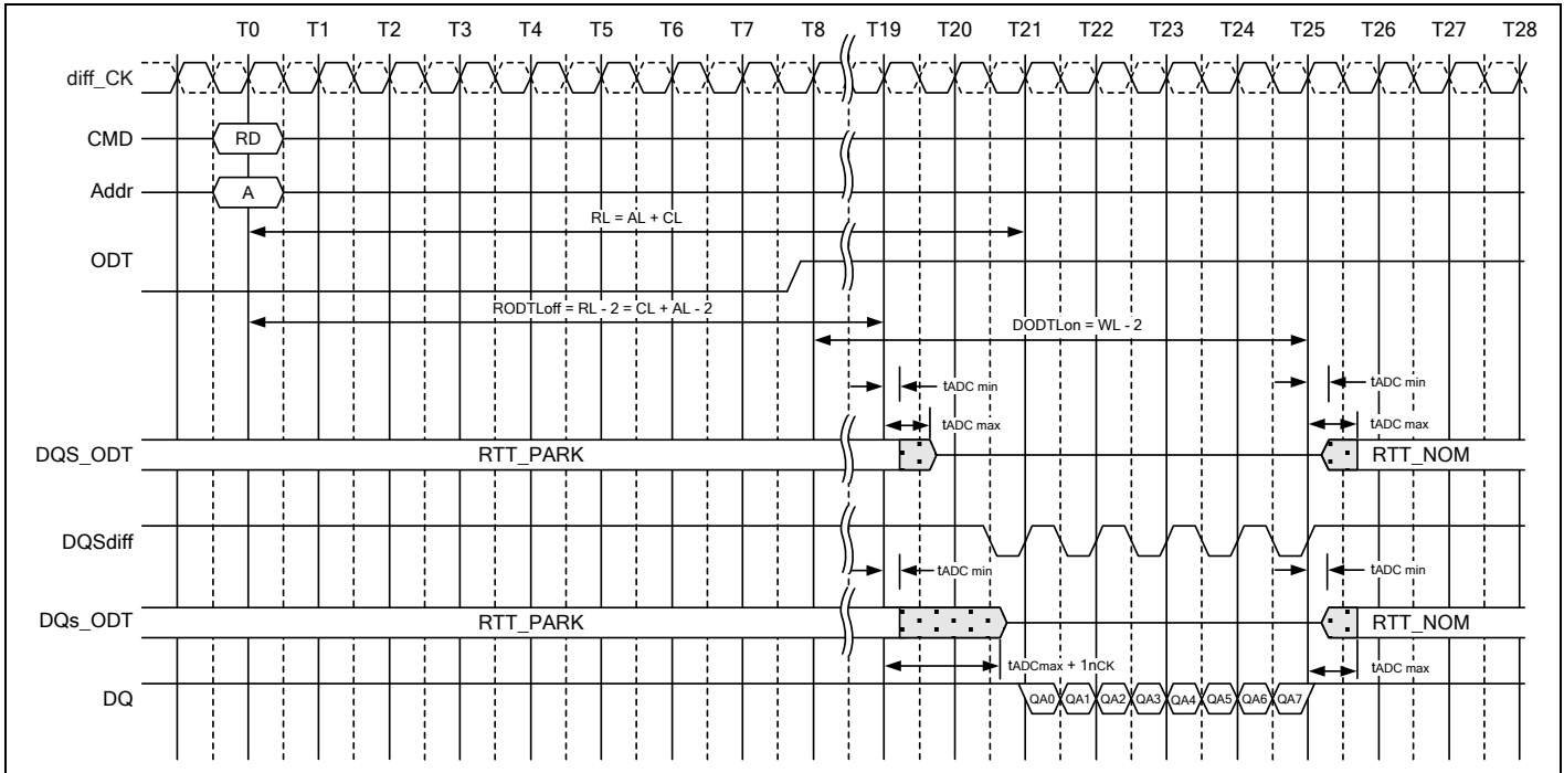
Figure 165 – Example: CL=11, PL=0; AL=CL-1=10; RL=AL+PL+CL=21; CWL=9; DODTLon=AL+CWL-2=17; RODTLoft=CL+AL-2=19; 1tCK preamble
