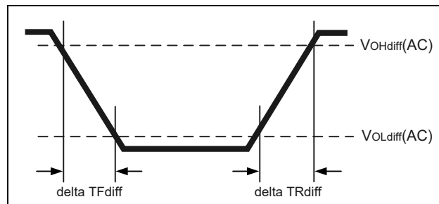
Figure 192 – Differential Output Slew Rate Definition
