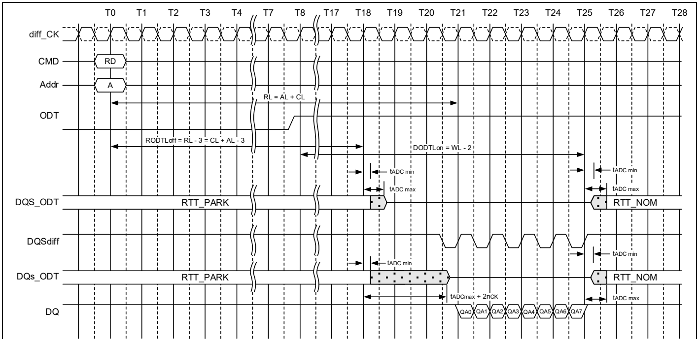
Figure 166 – Example: CL=11, PL=0; AL=CL-1=10; RL=AL+PL+CL=21; CWL=9; DODTLon=AL+CWL-2=17; RODTLoft=CL+AL-3=18; 2tCK preamble
