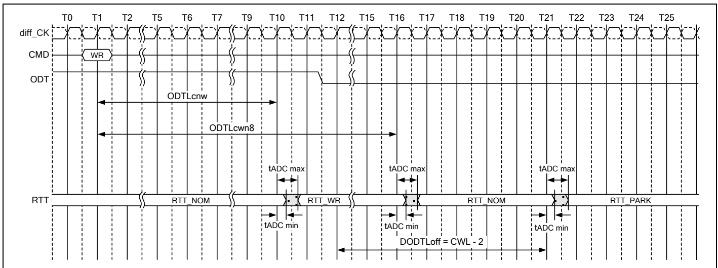
Figure 168 – Dynamic ODT overlapped with RTT_NOM (CL=14, CWL=11, BL=8, AL=0, CRC Disabled)
