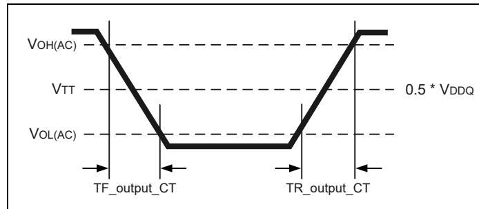
Figure 193 – Output Slew Rate Definition of Connectivity Test Mode
