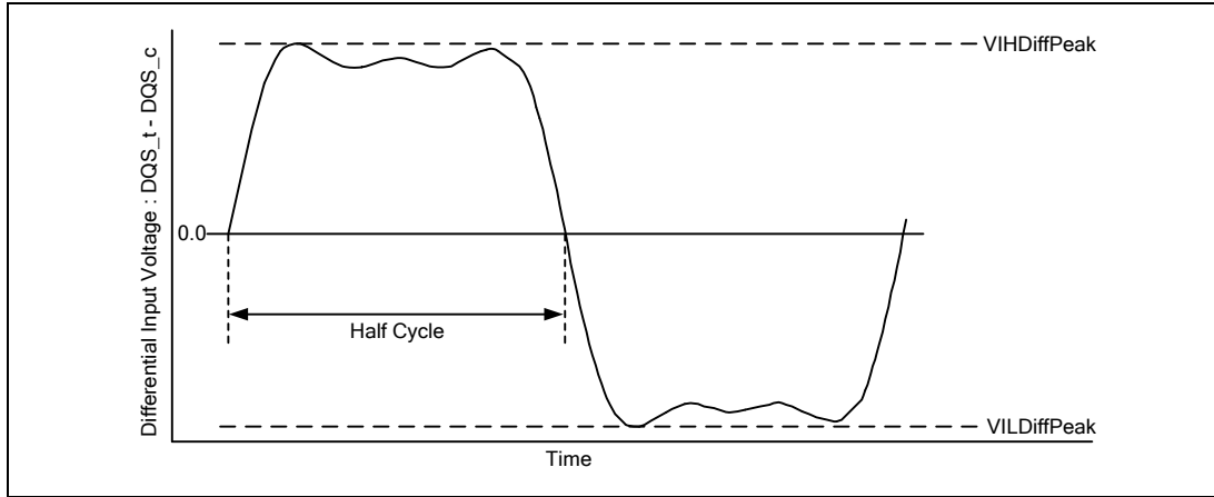
Figure 186 – Definition of differential DQS Signal AC-swing Level
