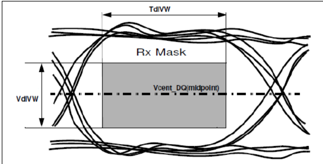
Figure 198 – DQ Receiver (Rx) compliance mask
