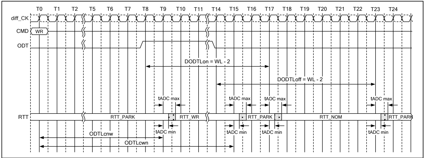
Figure 167 – ODT timing (Dynamic ODT, 1tCK preamble, CL=14, CWL=11, BL=8, AL=0, CRC Disabled)
