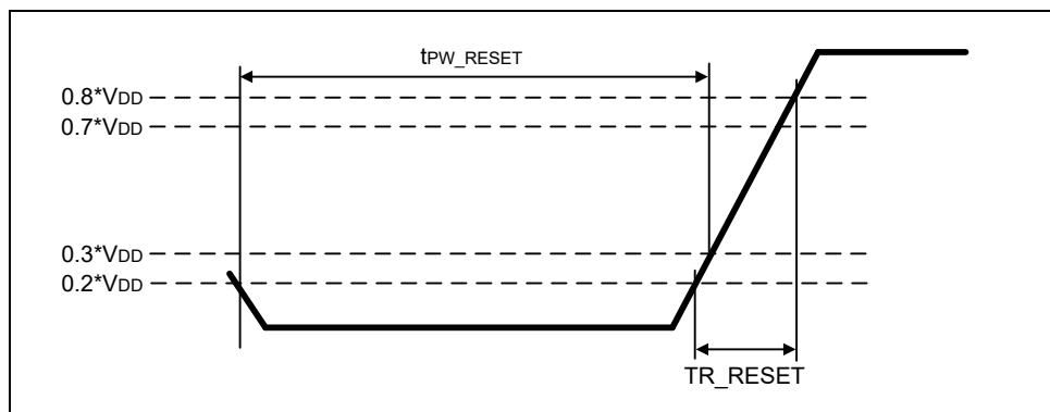
Figure 185 – RESET_n Input Slew Rate Definition
