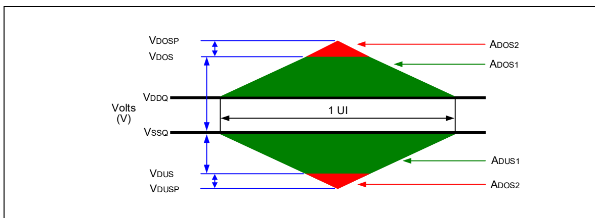
Figure 181 – Data, Strobe and Mask Overshoot and Undershoot Definition
