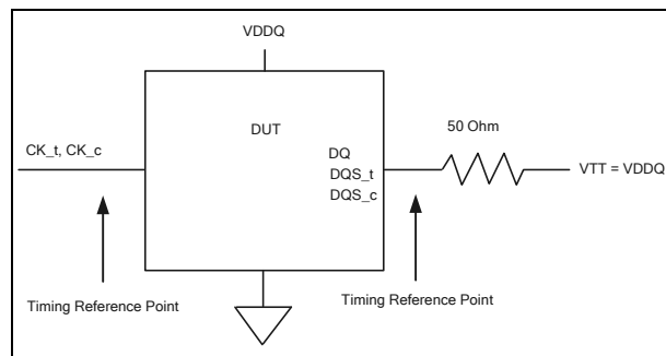
Figure 197 – Reference Load for AC Timing and Output Slew Rate
