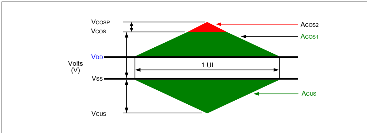
Figure 180 – Clock Overshoot and Undershoot Definition
