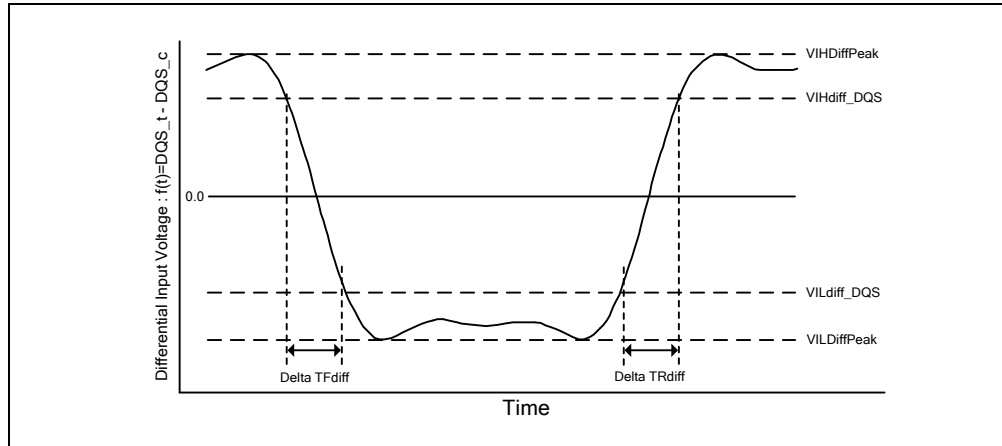
Figure 189 – Differential Input Slew Rate Definition for DQS t , DQS c
