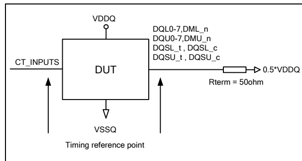
Figure 194 – Connectivity Test Mode Timing Reference Load
