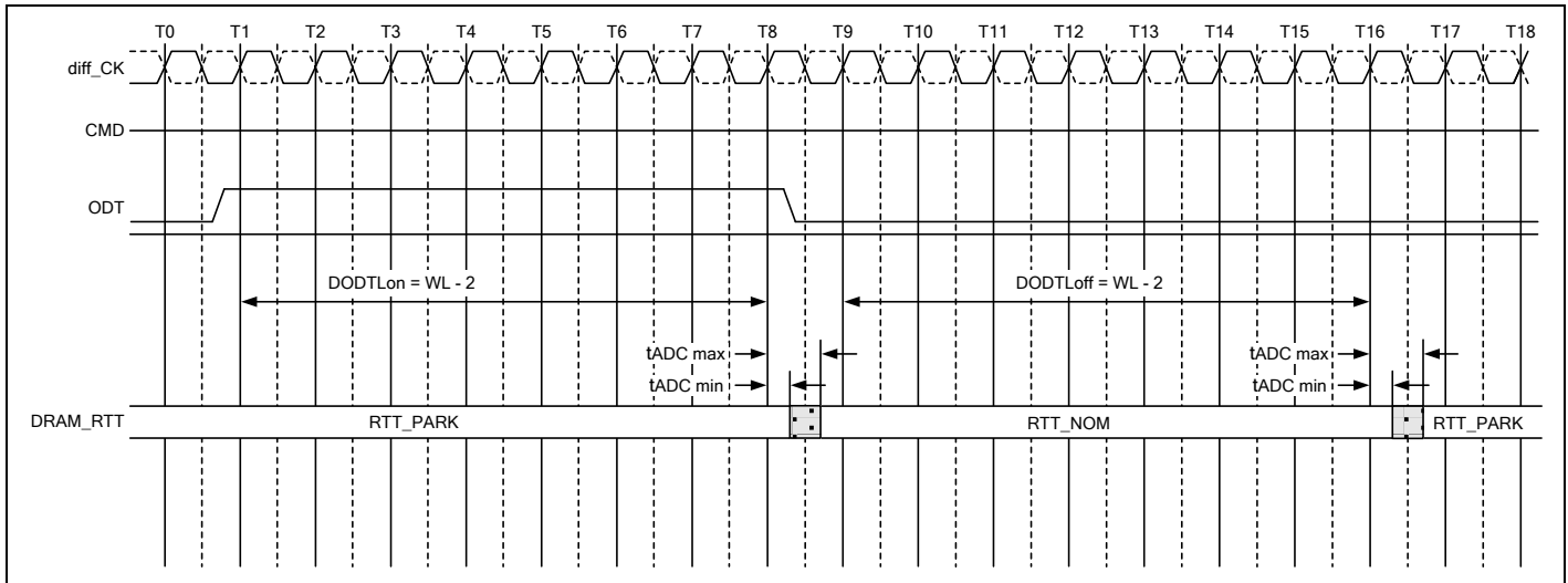
Figure 163 – Synchronous ODT Timing Example for CWL=9, AL=0, PL=0; DODTLon=WL-2=7 ; DODTLoff=WL-2=7
