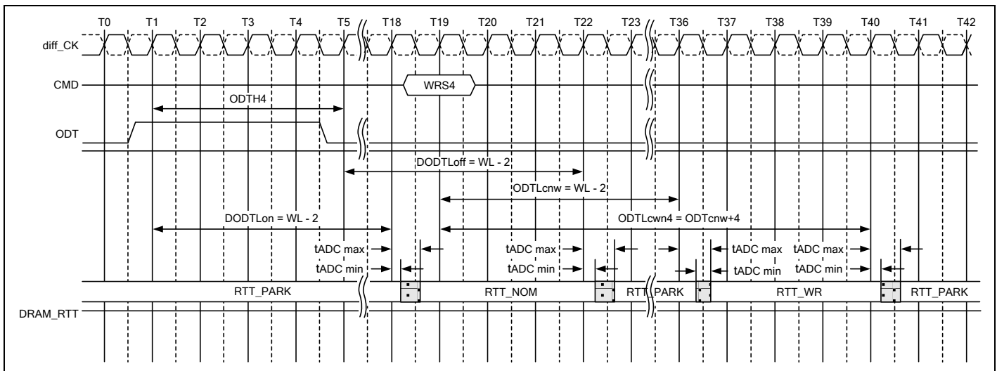
Figure 164 – Synchronous ODT example with BL=4, CWL=9, AL=10, PL=0; DODTLon/off=WL-2=17 , ODTCnw=WL-2=17
