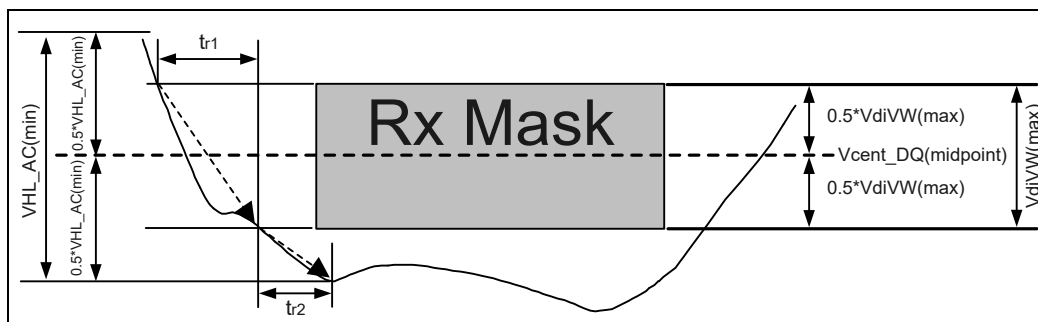
Figure 202 – Slew Rate Conditions for Falling Transition
