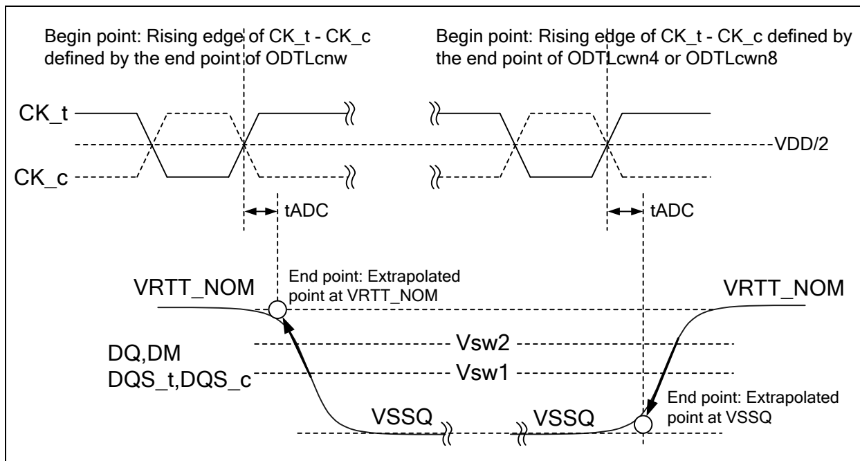
Figure 174 – Definition of tADC at Dynamic ODT Control
