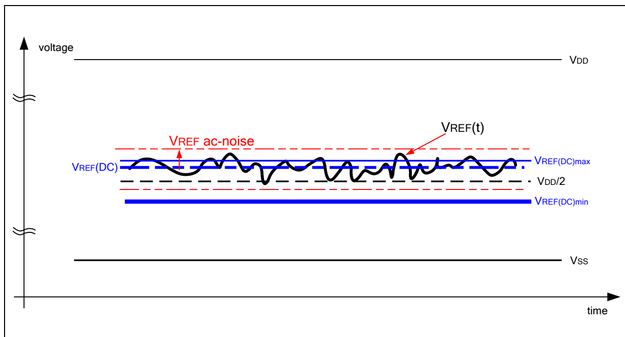
Figure 176 – Illustration of VREF(DC) tolerance and VREF AC-noise limits
