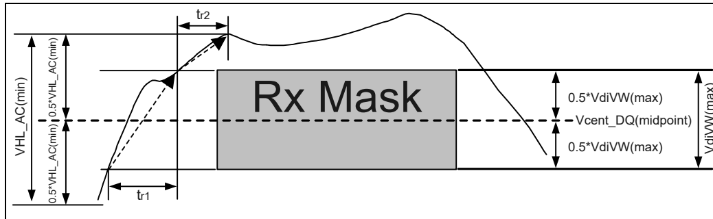
Figure 201 – Slew Rate Conditions for Rising Transition
