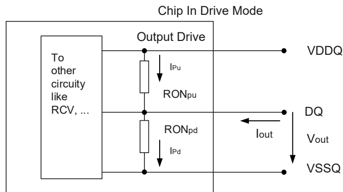
Figure 190 – Output driver
