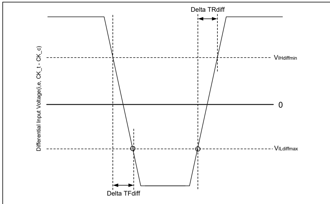
Figure 182 – Differential Input Slew Rate Definition for CK t , CK c
