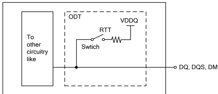
Figure 161 – Functional Representation of ODT
