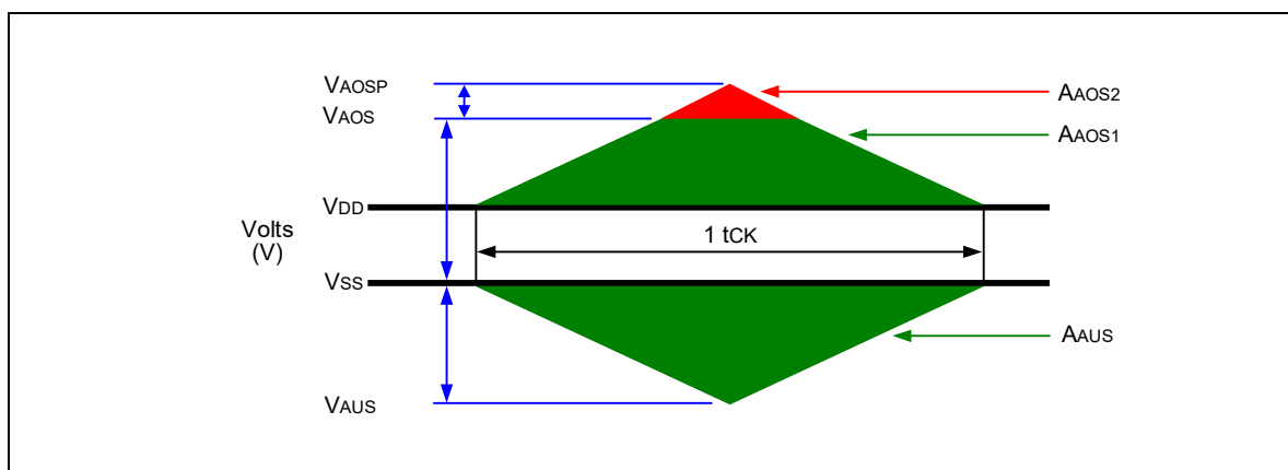
Figure 179 – Address, Command and Control Overshoot and Undershoot Definition
