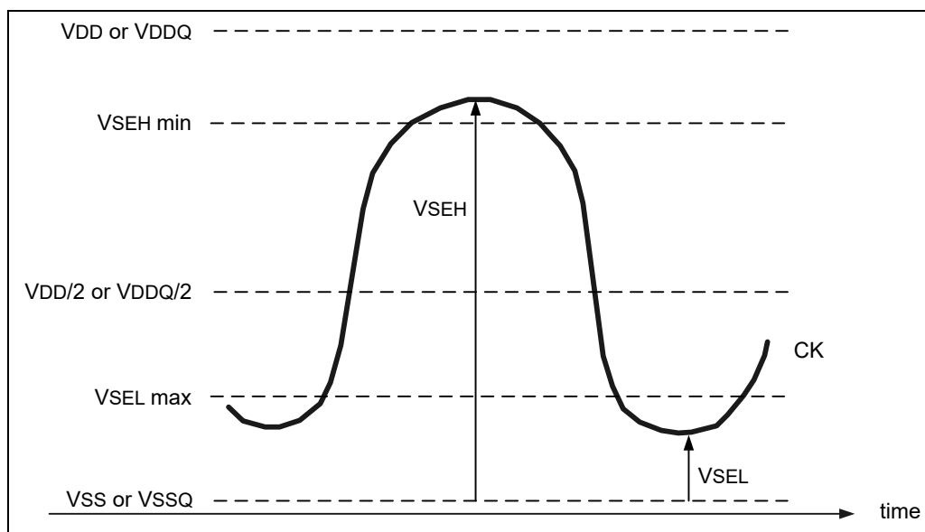
Figure 178 – Single-ended requirement for differential signals
