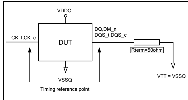
Figure 172 – ODT Timing Reference Load
