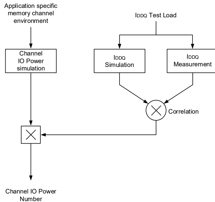
Figure 196 – Correlation from simulated Channel IO Power to actual Channel IO Power supported by I_{DDQ} Measurement
