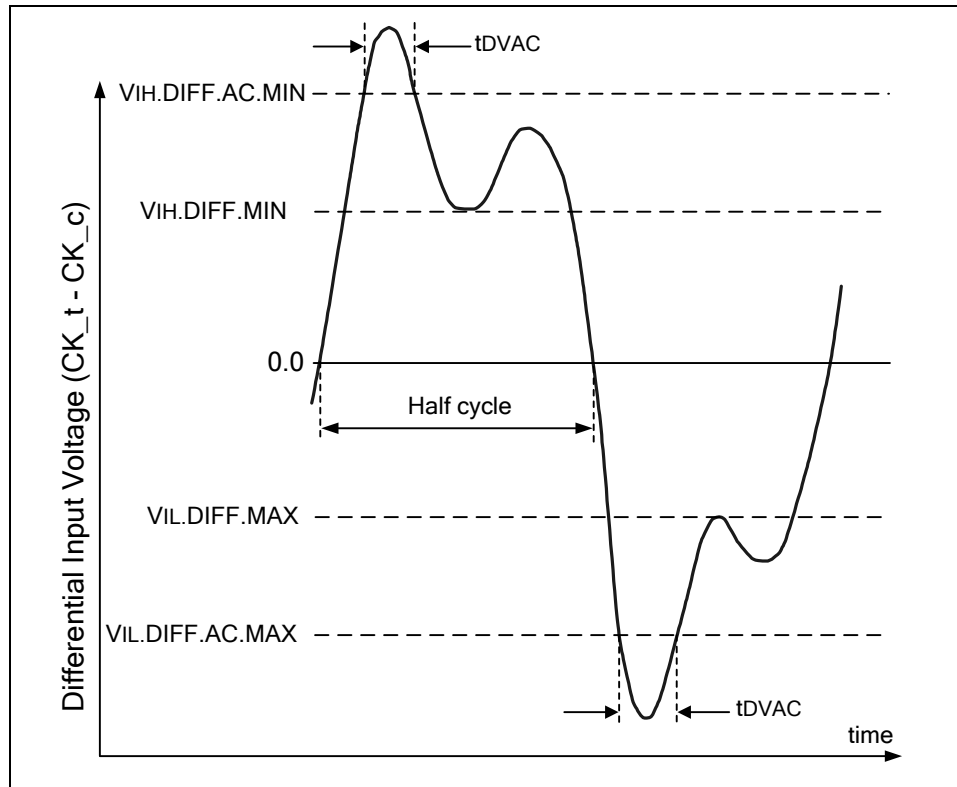
Figure 177 – Definition of differential ac-swing and “time above ac-level” tdVAC
