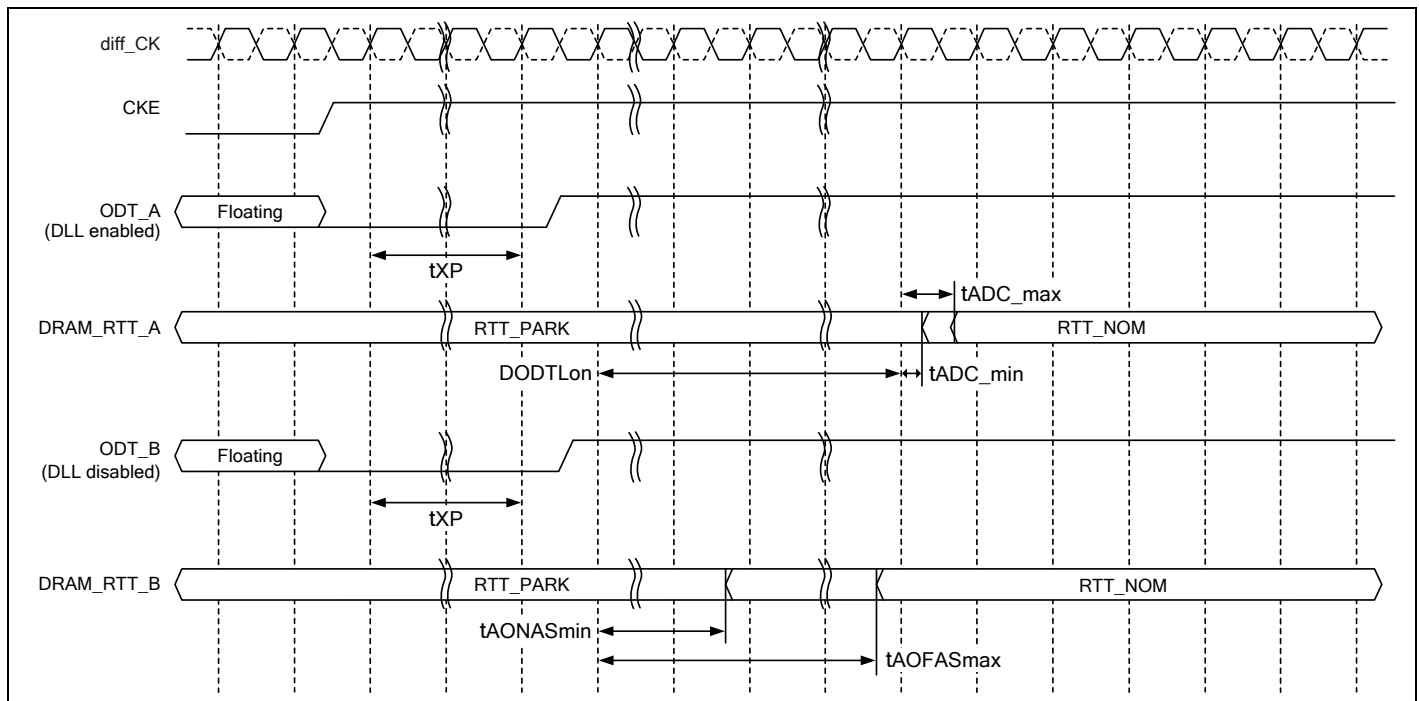
Figure 171 – ODT timing for power down exit with ODT buffer disable mode
