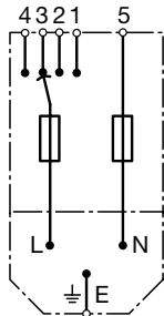
with internal connections Voltage Selector 4-positions, 2-pole
