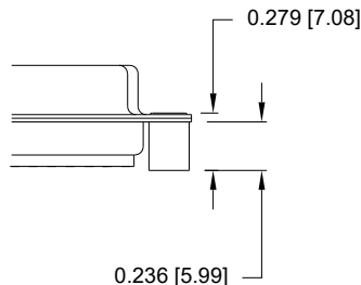
#4-40 INTERNAL THREADS
