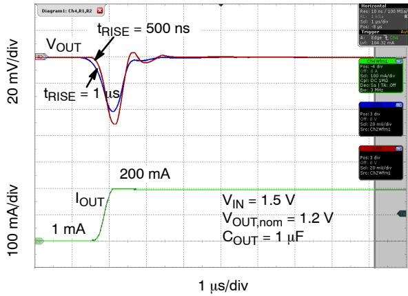
Figure 33. Load Transient Response, I_{OUT} = 1 \text{ mA} to 200 mA
