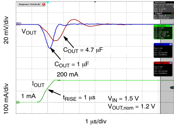
Figure 31. Load Transient Response, I_{OUT} = 1 \text{ mA} to 200 mA
