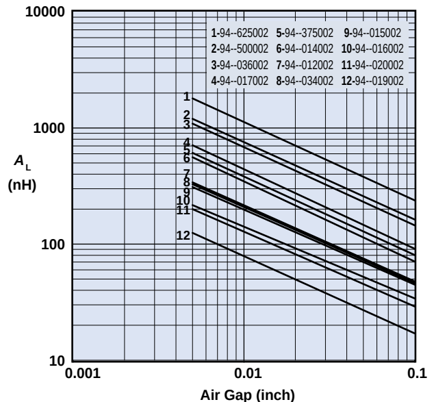
Figure 4 A_L vs. gap for E cores in 77 and 78 material.
