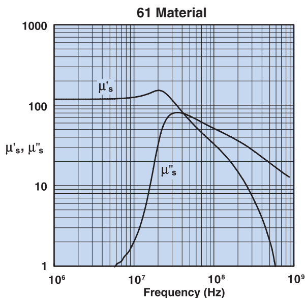
Figure 11 Complex Permeability vs. Frequency Measured on a 17/10/6mm toroid using the HP 4284A and the HP 4291A
