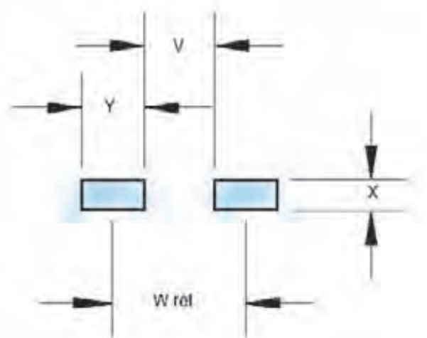
Land Pattern
