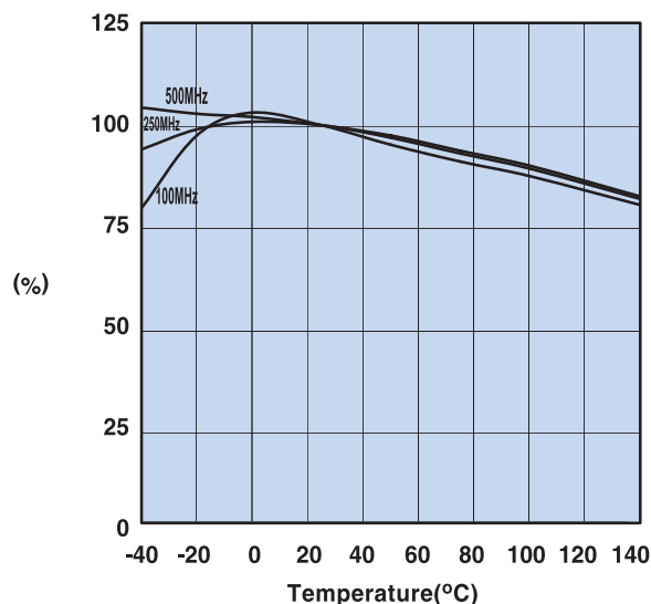
Figure 17 Percent of Original Impedance vs. Temperature Measured on a 2661000301 using the HP4291A.
