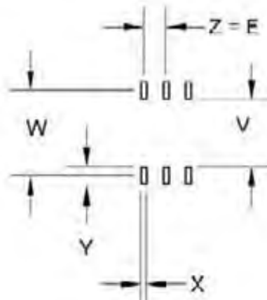
Land Pattern
