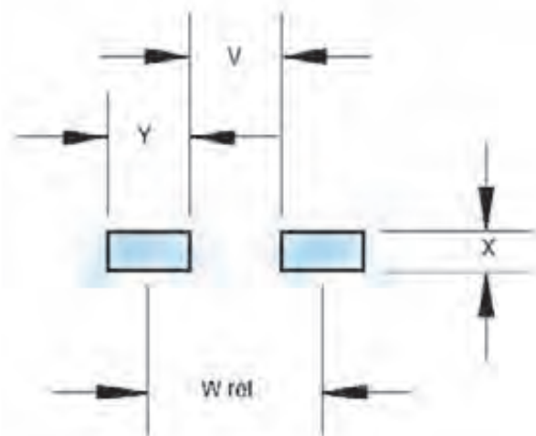
Land Pattern
