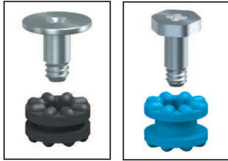
ROUND HEAD Screw supplied unassembled with isolator HEX HEAD
