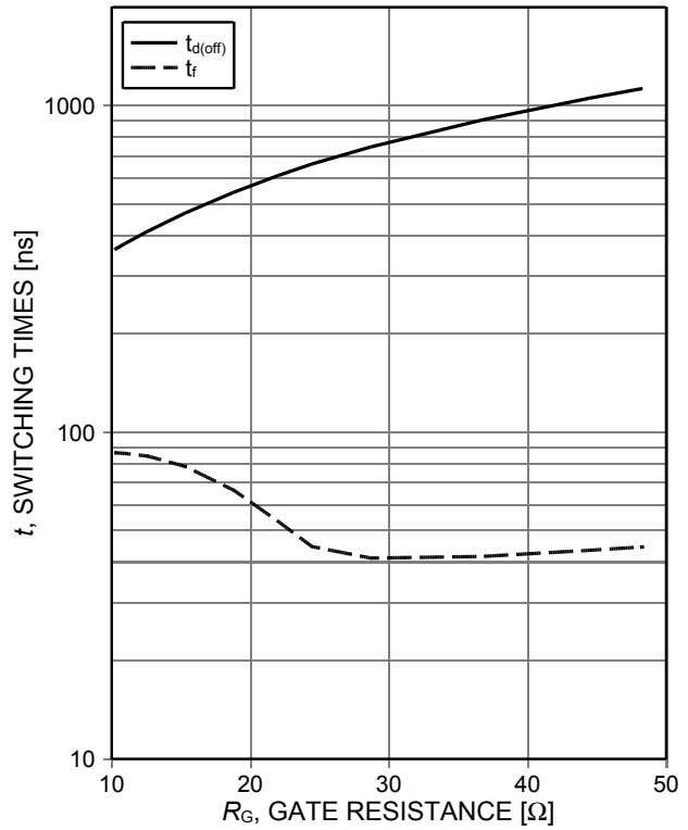
Figure 10. Typical switching times as a function of gate resistance (ind. load, T_j=175^\circ\text{C} , V_{\text{CE}}=600\text{V} , V_{\text{GE}}=0/15\text{V} , I_C=20\text{A} , test circuit in Fig. E)
