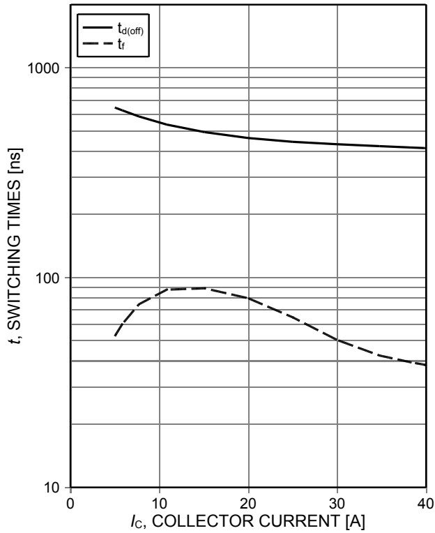
Figure 9. Typical switching times as a function of collector current (ind. load, T_j=175^\circ\text{C} , V_{\text{CE}}=600\text{V} , V_{\text{GE}}=0/15\text{V} , R_{\text{G(on)}}=15\Omega , R_{\text{G(off)}}=15\Omega , test circuit in Fig. E)
