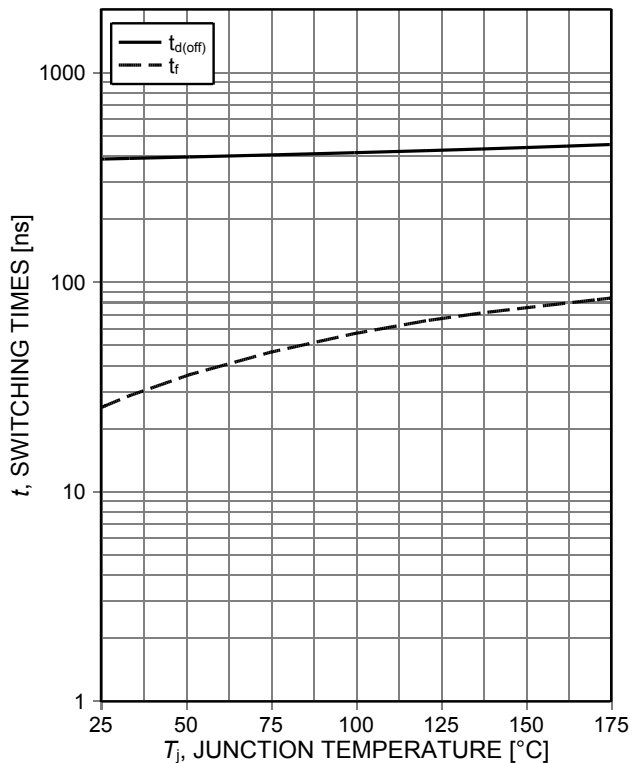
Figure 11. Typical switching times as a function of junction temperature (ind. load, V_{\text{CE}}=600\text{V} , V_{\text{GE}}=0/15\text{V} , I_C=20\text{A} , R_{\text{G(on)}}=15\Omega , R_{\text{G(off)}}=15\Omega , test circuit in Fig. E)
