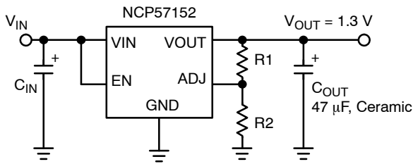
Figure 1. Adjustable Regulator
