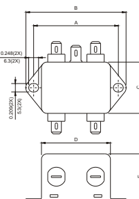
SUGGESTED MOUNTING CUTOUT
