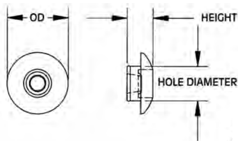
FEMALE RIVET
