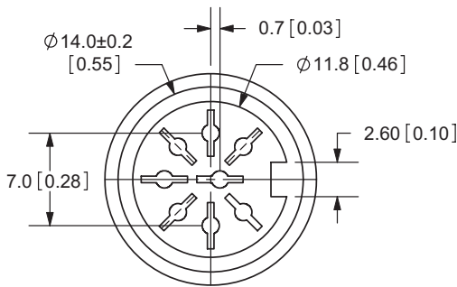
SD-30BV
