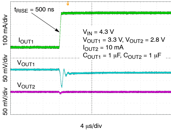
Figure 48. Load Transient Response – 3.3 V – Rising Edge, I_{OUT1} = 1 \text{ mA} to 300 \text{ mA}
