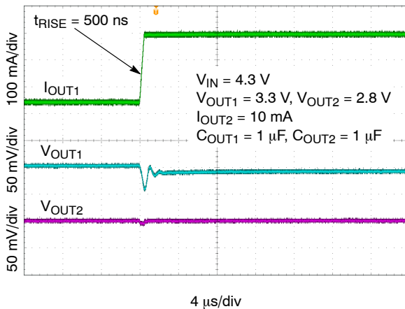
Figure 50. Load Transient Response – 3.3 V – Rising Edge, I_{OUT1} = 50 \text{ mA} to 300 \text{ mA}
