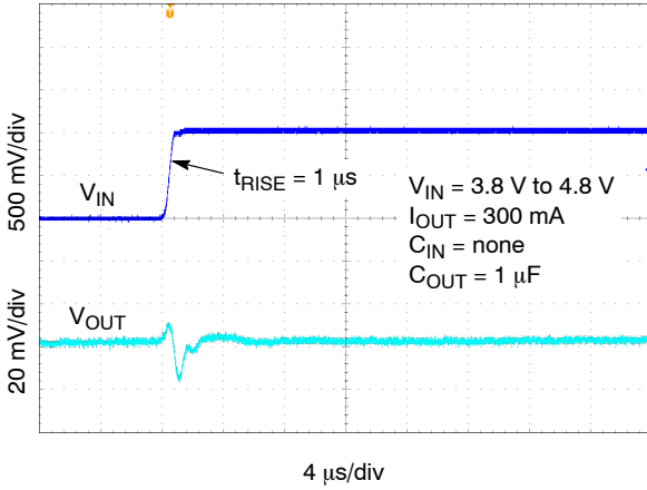
Figure 36. Line Transient Response– Rising Edge, V_{OUT} = 3.3 V, I_{OUT} = 300 mA
