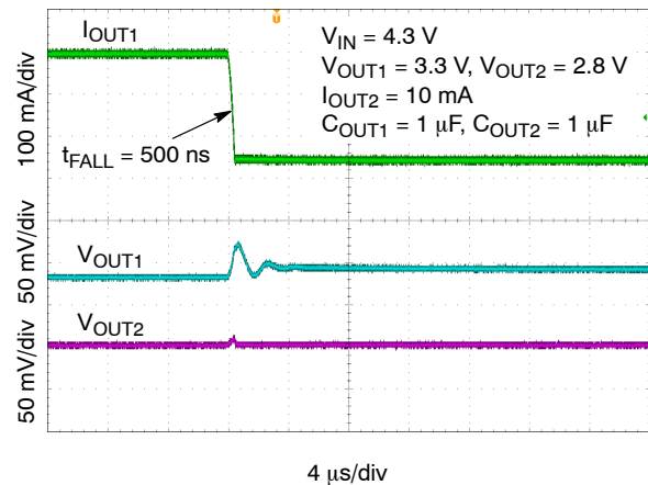
Figure 51. Load Transient Response – 3.3 V – Falling Edge, I_{OUT1} = 300 \text{ mA} to 50 \text{ mA}
