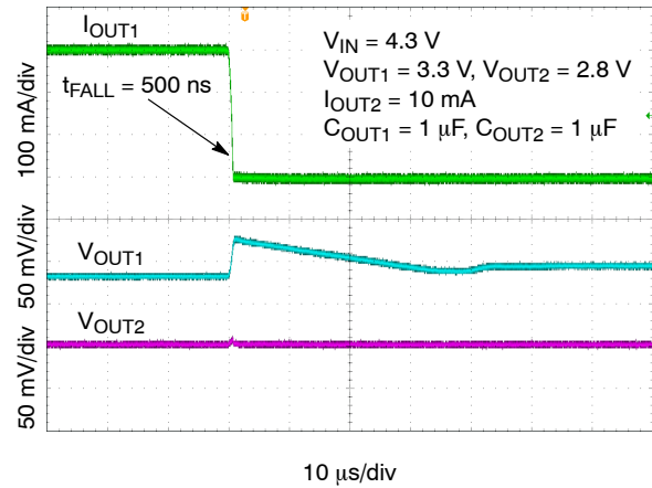
Figure 49. Load Transient Response – 3.3 V – Falling Edge, I_{OUT1} = 300 \text{ mA} to 1 \text{ mA}
