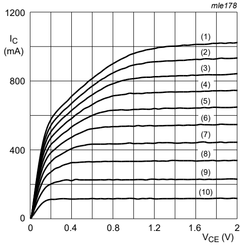
T_{amb} = 25\text{ }^\circ\text{C} (1) I_B = 2600\text{ }\mu\text{A} (2) I_B = 2340\text{ }\mu\text{A} (3) I_B = 2080\text{ }\mu\text{A} (4) I_B = 1820\text{ }\mu\text{A} (5) I_B = 1560\text{ }\mu\text{A} (6) I_B = 1300\text{ }\mu\text{A} (7) I_B = 1040\text{ }\mu\text{A} (8) I_B = 780\text{ }\mu\text{A} (9) I_B = 520\text{ }\mu\text{A} (10) I_B = 260\text{ }\mu\text{A}
