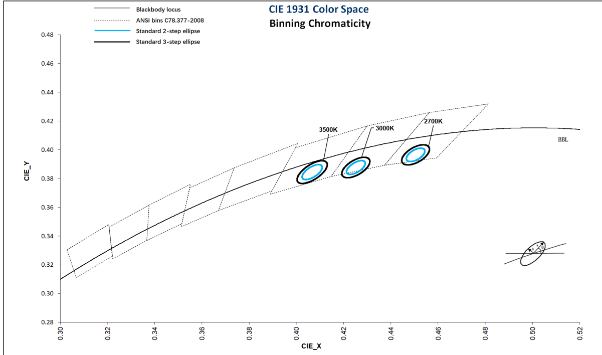
Chromaticity Binning Diagram 1 - TC62 Sensus (BBBL)
