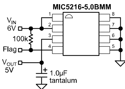
5V Low-Noise Regulator
