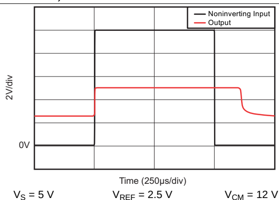
Figure 20. Noninverting Differential Input Overload
