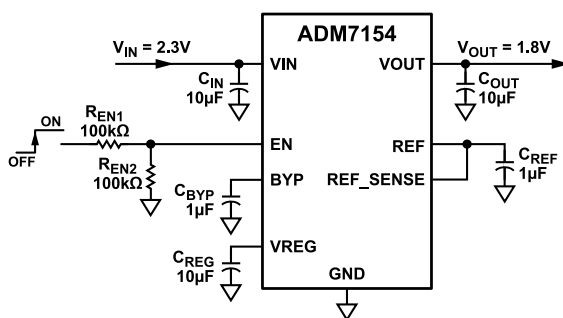
Figure 52. Typical EN Pin Voltage Divider
