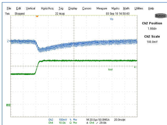
Figure 27: Transient Response, 24.5A to 35A step (2.5A/us)
