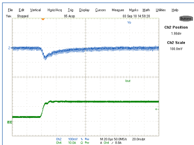
Figure 26: Transient Response, 3.5A to 14A step (2.5A/μs) Ch2: V_{out}
