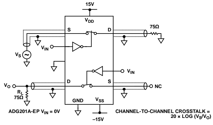
Figure 9. Channel-to-Channel Crosstalk
