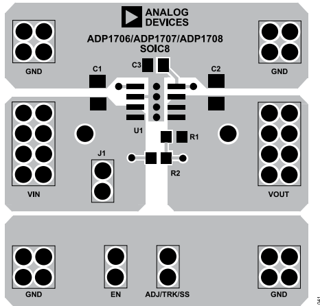
Figure 42. Example PCB Layout
