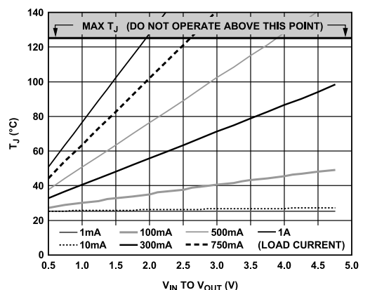
Figure 36. 500 mm 2 of PCB Copper, T_A = 25^\circ\text{C} , SOIC
