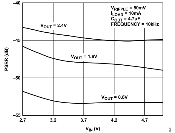
Figure 25. ADP1708 Power Supply Rejection Ratio (PSRR) vs. Input Voltage ( V_{IN} )
