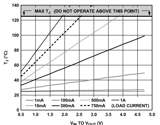
Figure 37. 100 mm 2 of PCB Copper, T_A = 25^\circ\text{C} , SOIC
