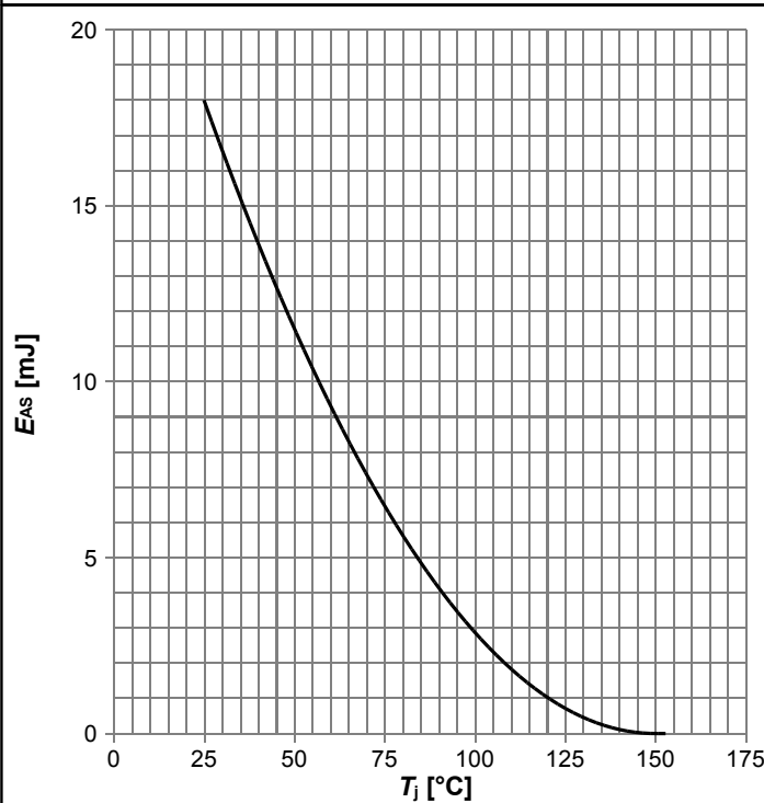
Diagram 11: Avalanche energy
