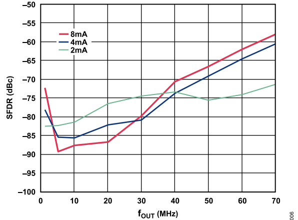
Figure 6. SFDR vs. f_{OUT} at Three I_{OUTFS} Values
