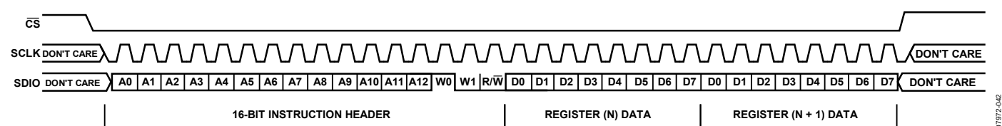
Figure 56. Serial Control Port Write—LSB First, 16-Bit Instruction, Two Bytes of Data
