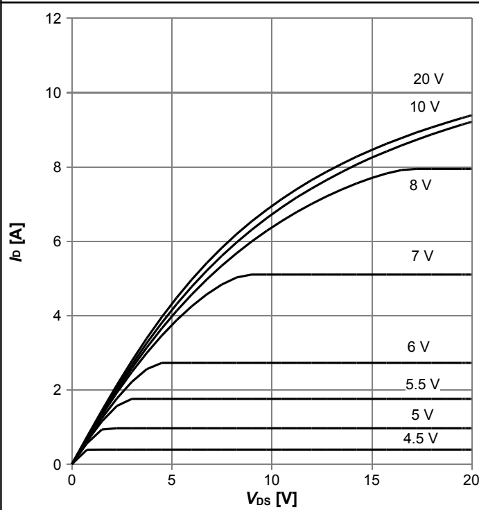
Typ. output characteristics
