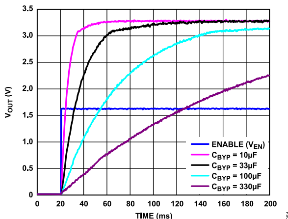
Figure 54. Typical Start-Up Behavior with C_{BYP} = 10 \mu\text{F} to 330 \mu\text{F}
