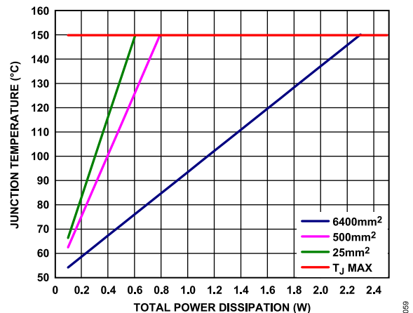
Figure 59. Junction Temperature vs. Total Power Dissipation for the 8-Lead SOIC, T_A = 50^\circ\text{C}
