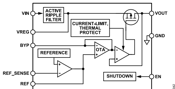
Figure 42. Simplified Internal Block Diagram
