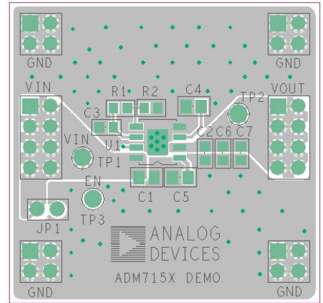
Figure 64. Example 8-Lead SOIC PCB Layout
