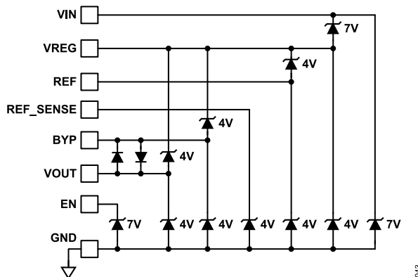
Figure 43. Simplified ESD Protection Block Diagram
