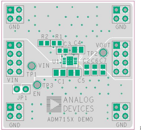
Figure 63. Example 8-Lead LFCSP PCB Layout
