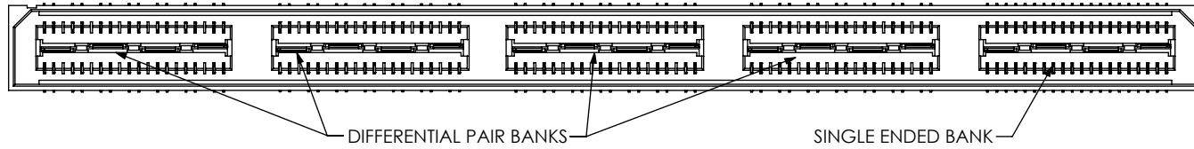
FIG 6 (**QSE-070-01-XXX-D-DP-A-DDDDS) (** = SEE NOTE 17)
