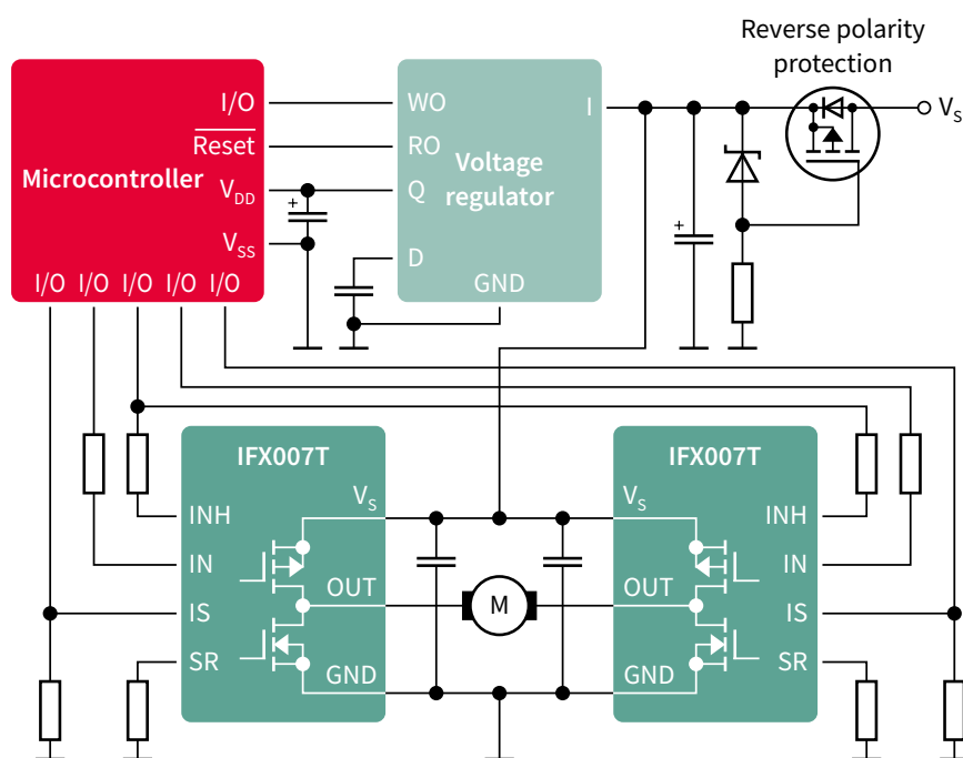
High current H-bridge
