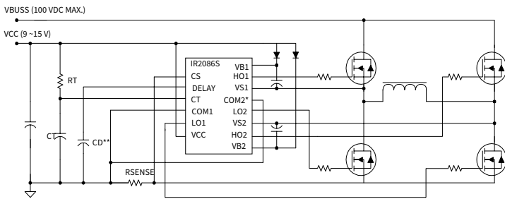
Typical connection
