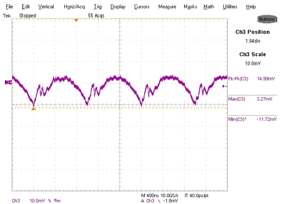
Figure 32: Output Voltage Ripple, 3A load Ch3: V out
