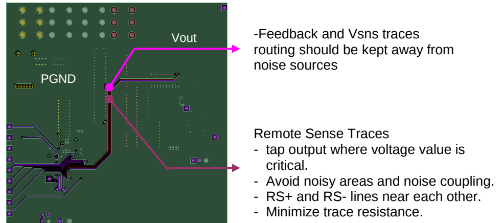
Figure 49e: IRDC3847 Demo board Layout Considerations – Mid Layer 3
