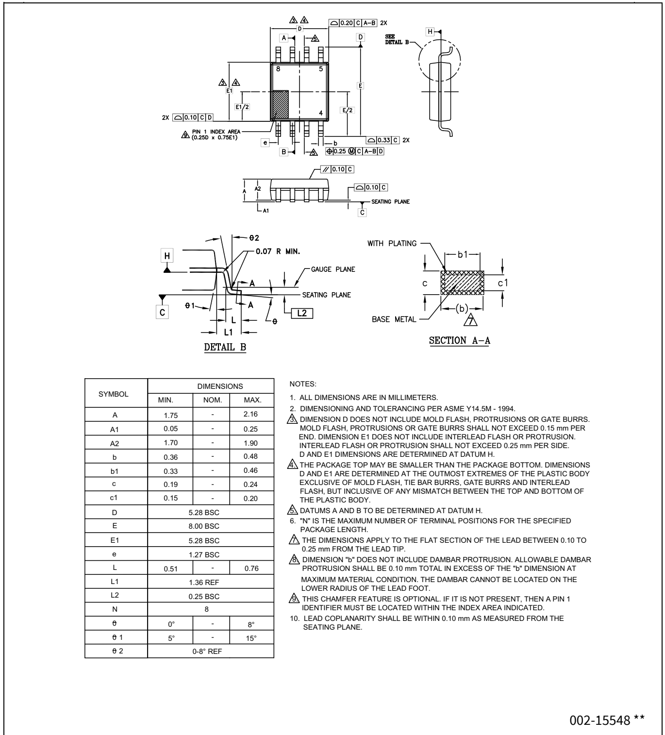
Figure 151 SOIC 8-lead, 208 mil body width (SOC008)
