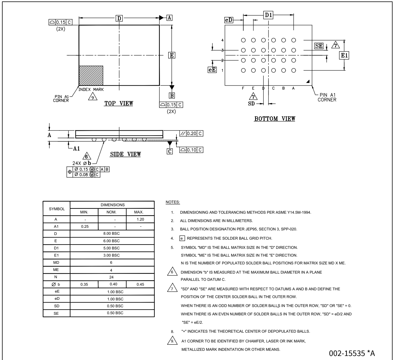
Figure 155 Ball grid array 24-ball 6 x 8 mm (FAC024)
