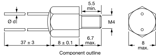
Component outline
