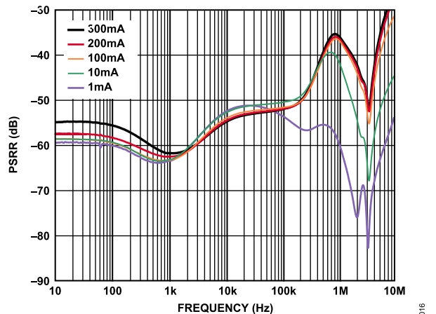
Figure 14. Power Supply Rejection Ratio vs. Frequency, V_{OUT} = 1.8 V
