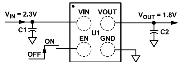
Figure 1. ADP172 with Fixed Output Voltage, 1.8 V
