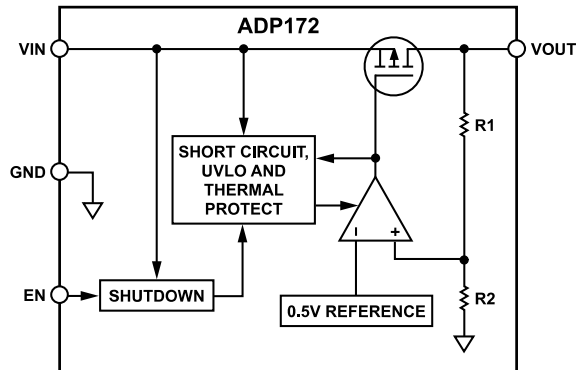
Figure 23. ADP172 Internal Block Diagram
