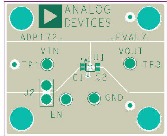
Figure 37. Example ADP172 PCB Layout
