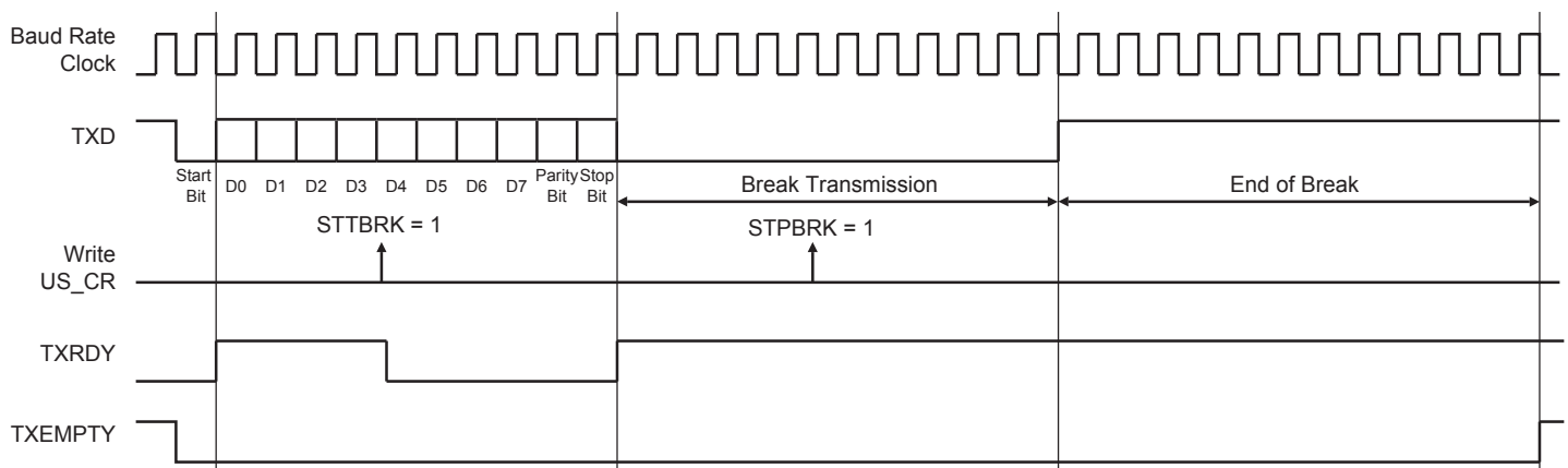
Figure 38-25: Break Transmission
