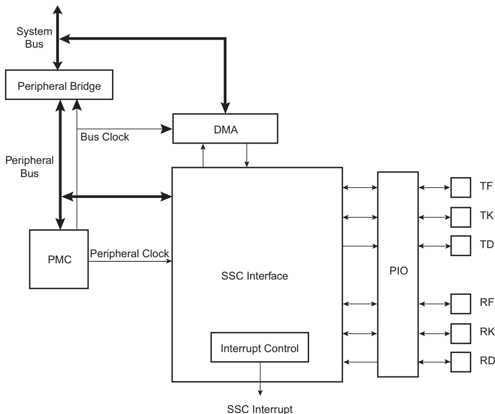
Figure 43-1: Block Diagram
