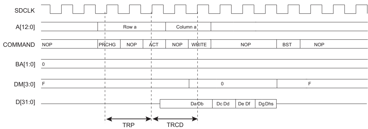
Figure 29-7: Burst Write Access, Row Closed, SDR-SDRAM Device
