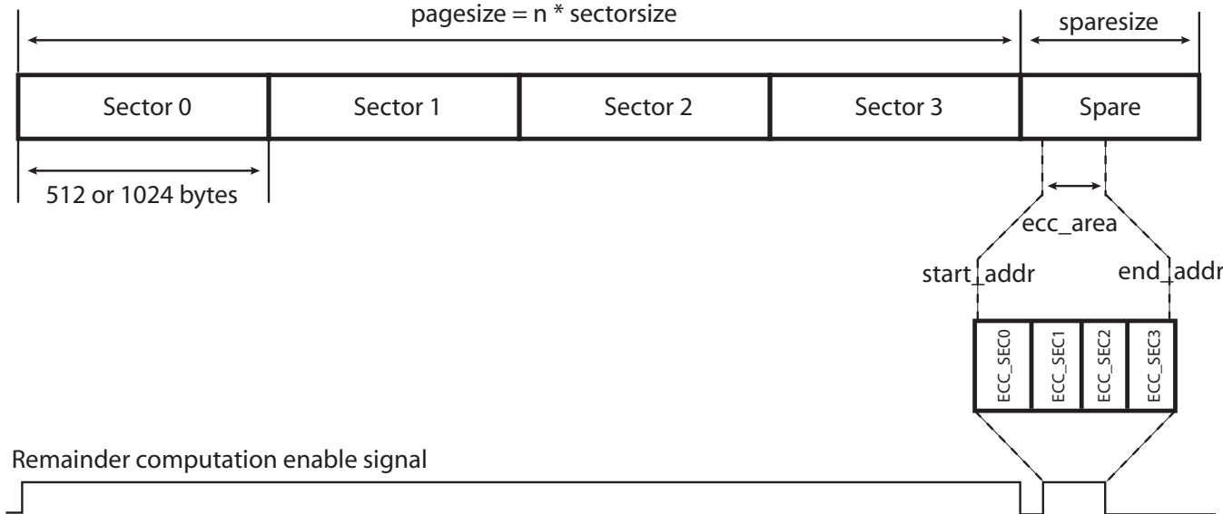
Figure 26-6: Read Operation Read NAND operation with SPAREEN set to Zero and AUTO set to One
