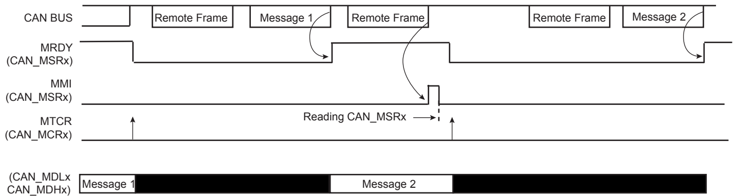
Figure 40-17: Producer Handling
