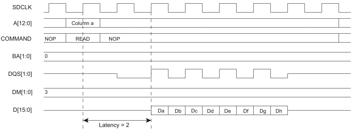
Figure 29-14: Burst Read Access, Latency = 2, Low-power DDR1-SDRAM Devices
