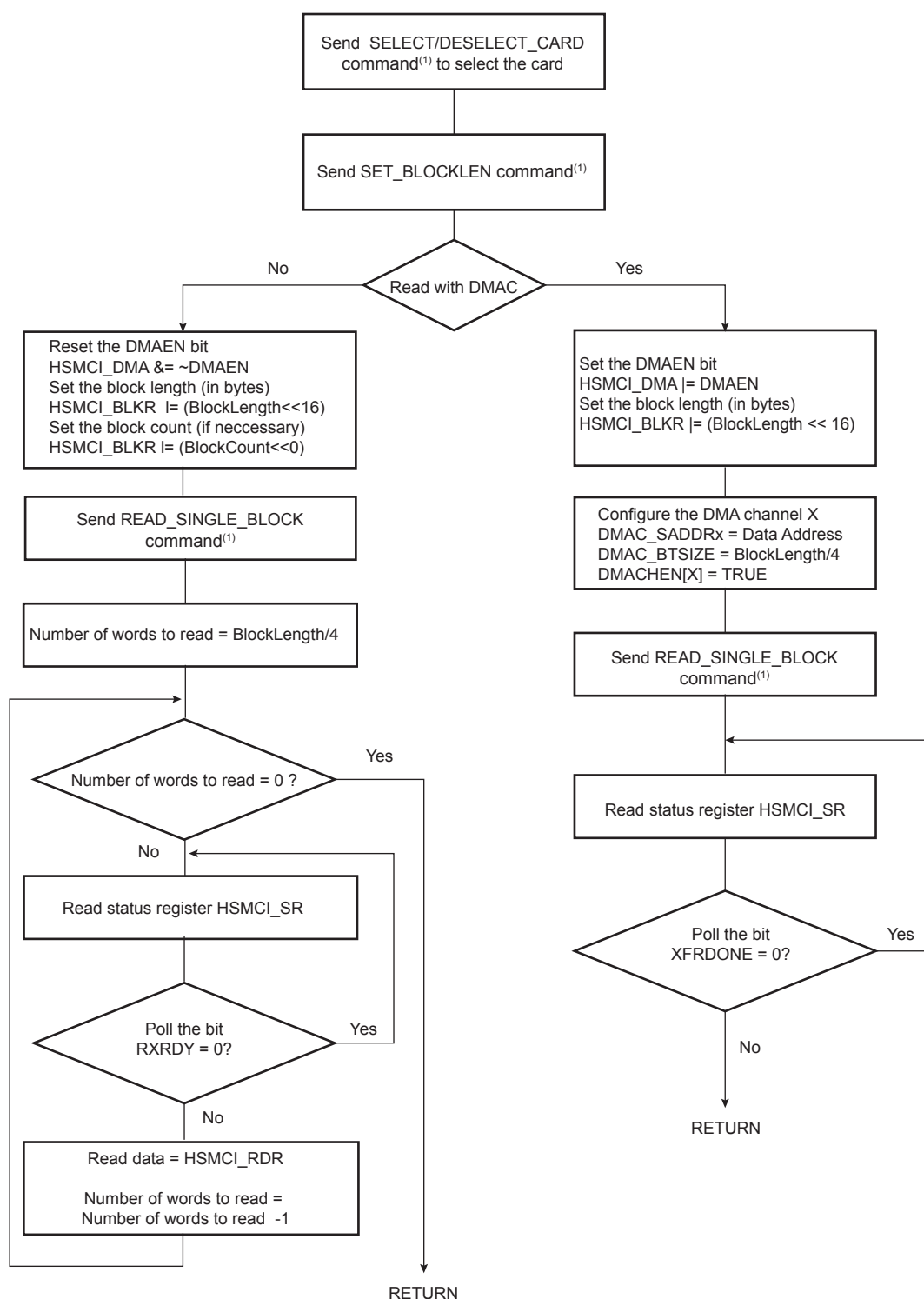
Figure 33-8: Read Functional Flow Diagram
