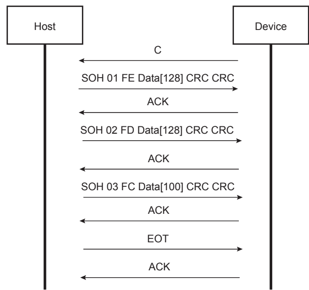
Figure 10-11: Xmodem Transfer Example
