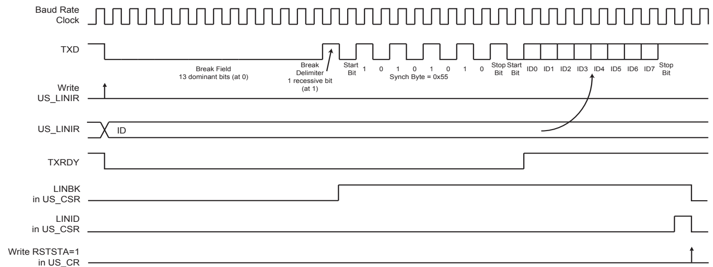
Figure 38-39: Header Transmission
