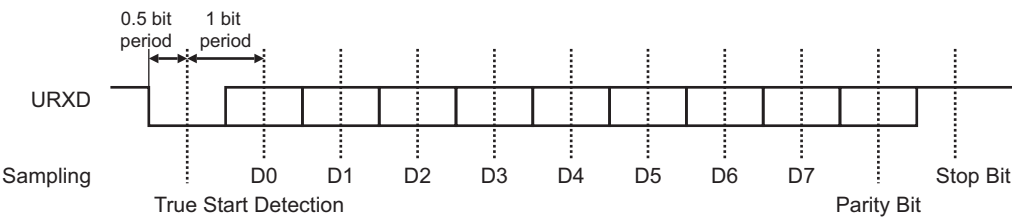
Figure 39-4: Character Reception
