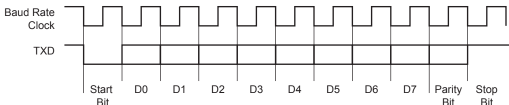
Figure 38-5: Character Transmit
