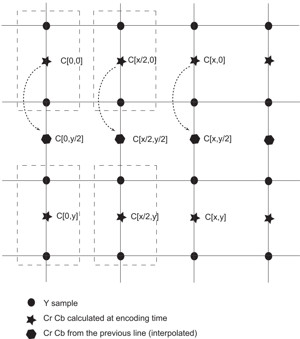
Figure 45-3: 4:2:2 Packed Memory Upsampling Algorithm Vertical and Horizontal upsampling 4:2:2 to 4:4:4 conversion 90 or 270 degree
