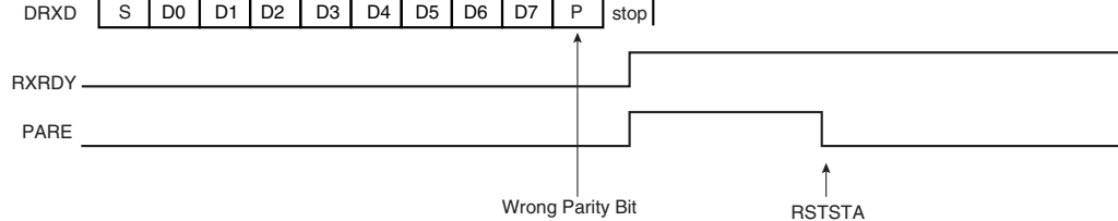
Figure 23-8: Parity Error
