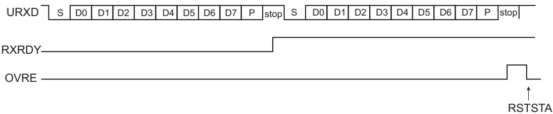
Figure 39-3: Start Bit Detection
