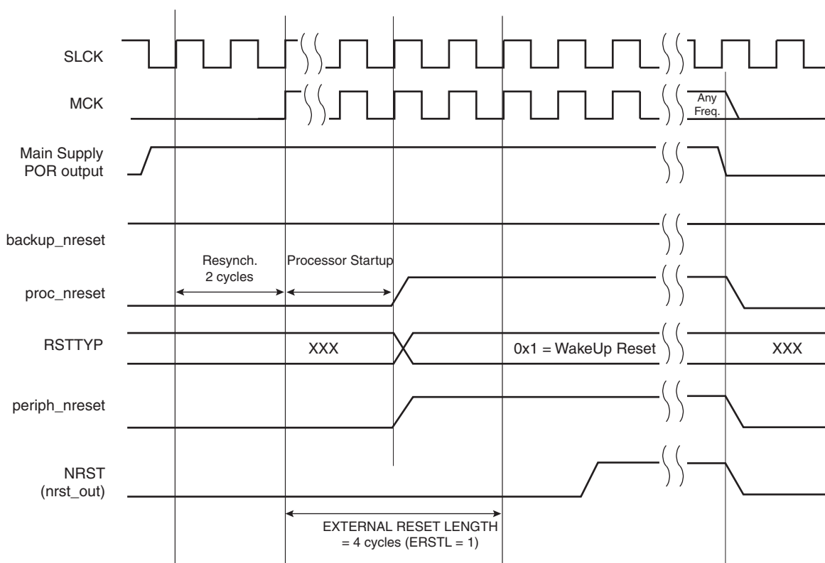
Figure 13-5: Wake-up Reset
