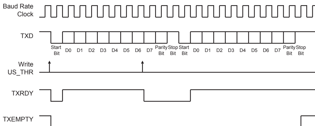
Figure 38-6: Transmitter Status
