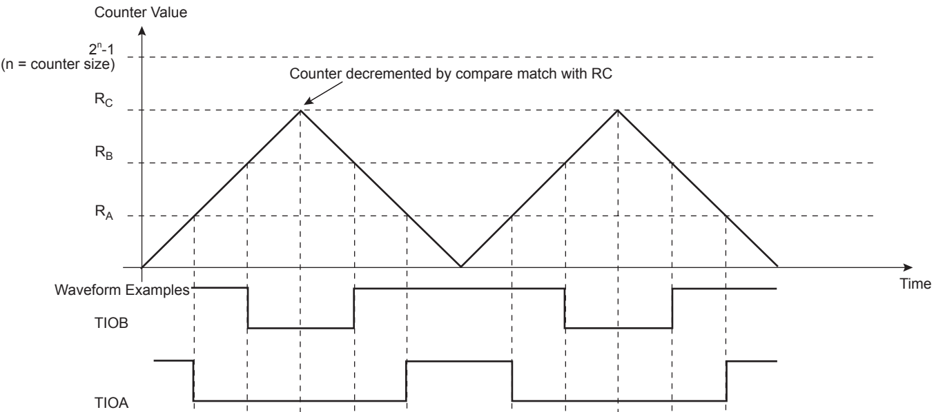
Figure 35-13: WAVSEL = 11 without Trigger
