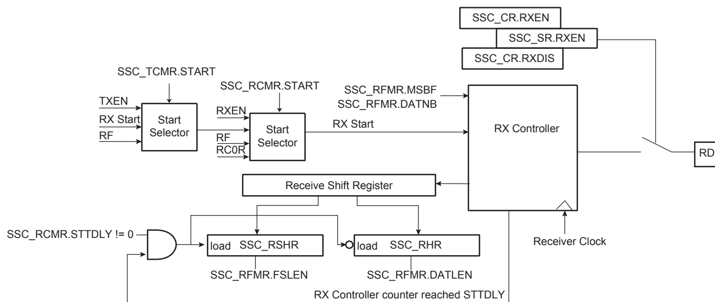
Figure 43-12: Receiver Block Diagram
