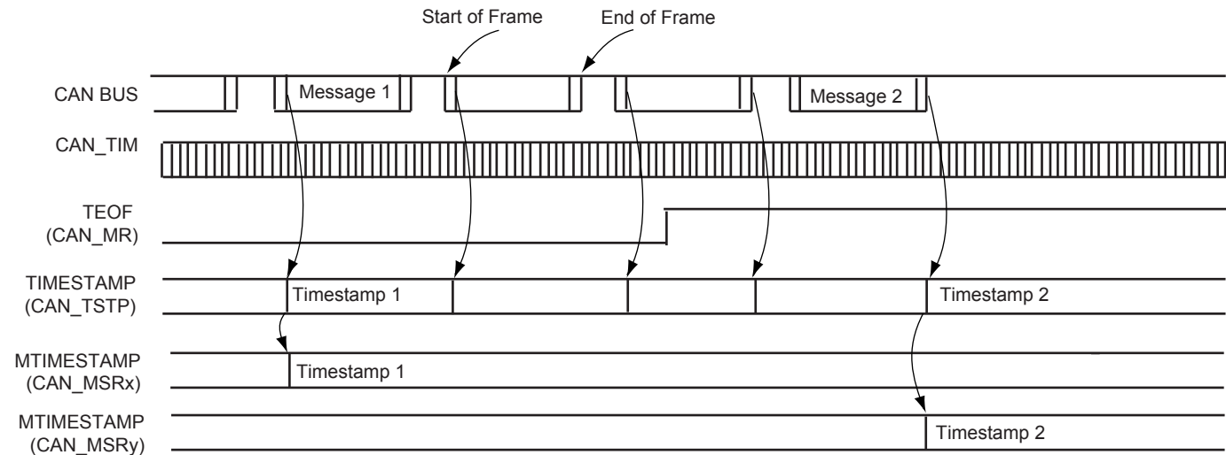
Figure 40-19: Mailbox Timestamp
