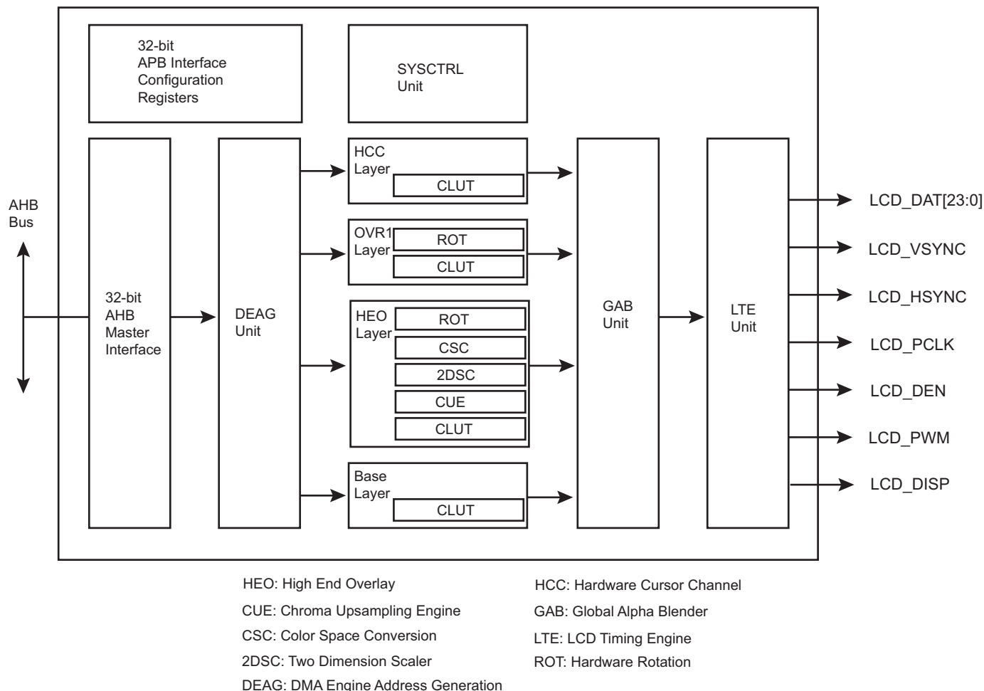
Figure 45-1: Block Diagram
