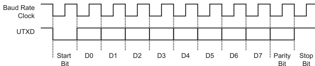
Figure 39-9: Character Transmission
