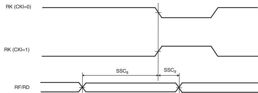
Figure 46-20: SSC Receiver, RK and RF in Input
