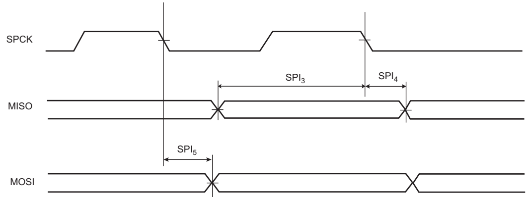
Figure 46-11: SPI Master Mode 0 and 3
