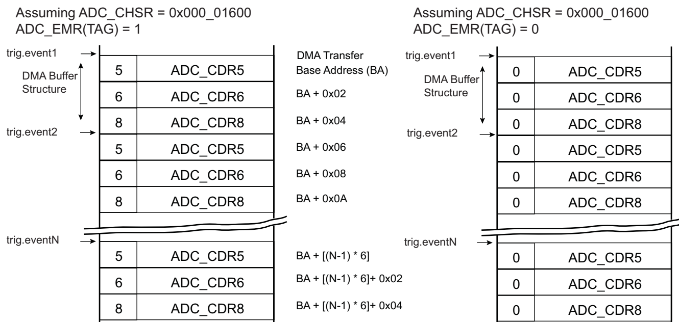
Figure 41-13: Buffer Structure
