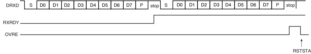
Figure 23-7: Receiver Overrun
