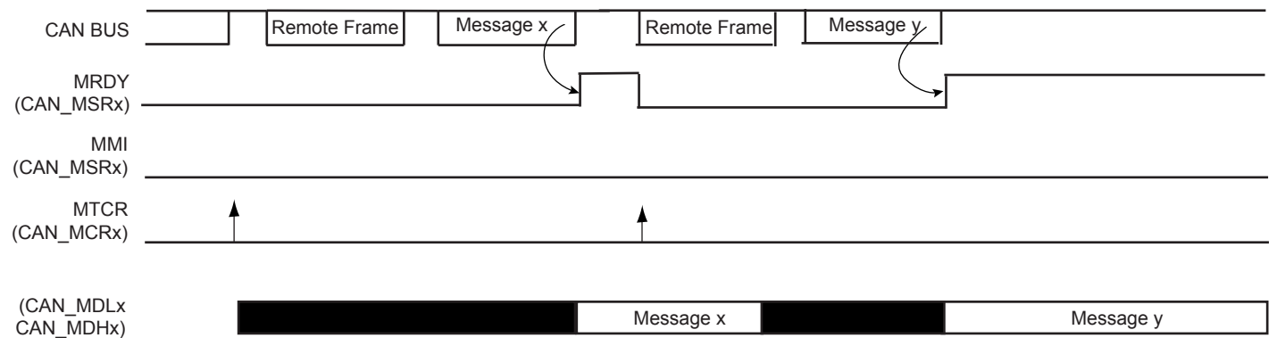
Figure 40-18: Consumer Handling
