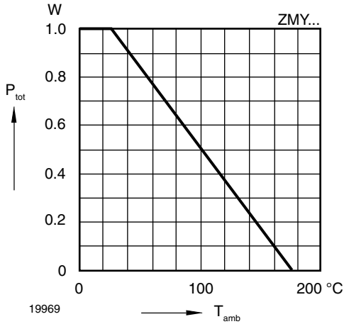
Fig. 1 - Admissible Power Dissipation vs. Ambient Temperature
