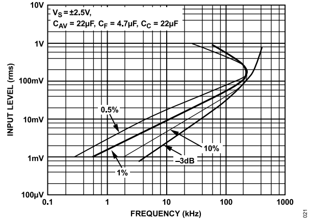
Figure 20. Error Contours Driving Pin 1
