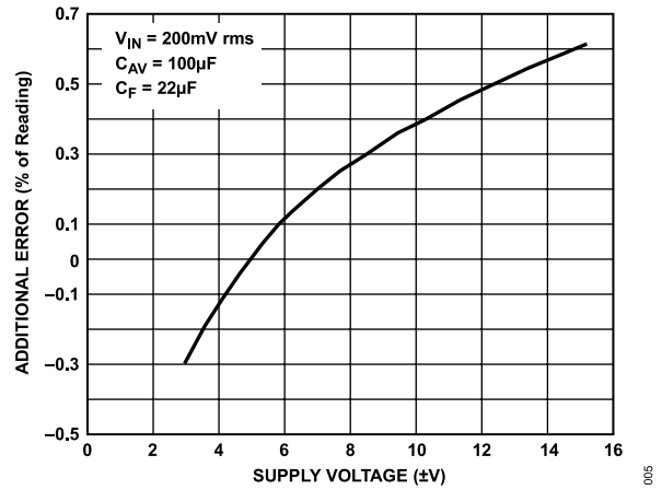
Figure 7. Additional Error vs. Supply Voltage
