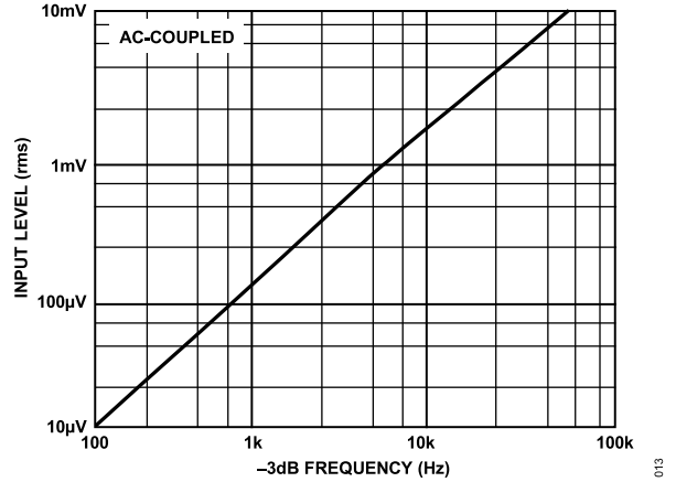
Figure 13. RMS Input Level vs. -3 dB Frequency; Negative DC Output
