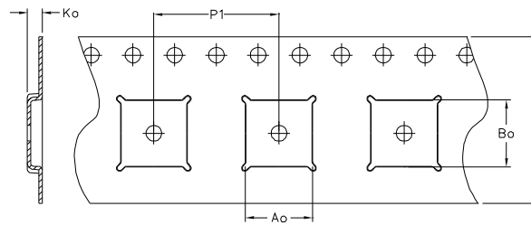
TAPE DIMENSIONS
