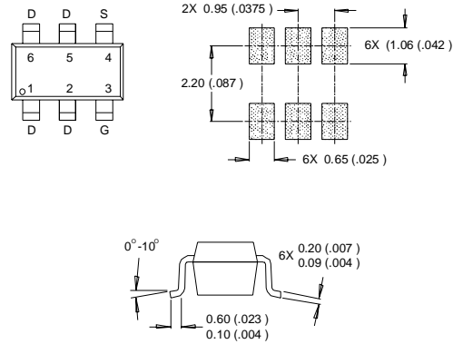
LEAD ASSIGNMENTS
