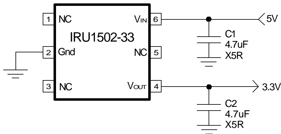
Figure 1 - Typical application of IRU1502-33.
