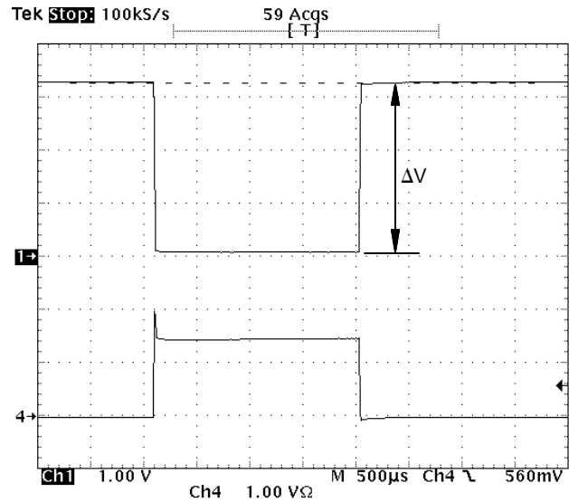
Figure 5 - Output short circuit operation. \Delta V = 3.26\text{V} Ch1: Output voltage, 1V/div Ch4: Load Current, 1A/div
