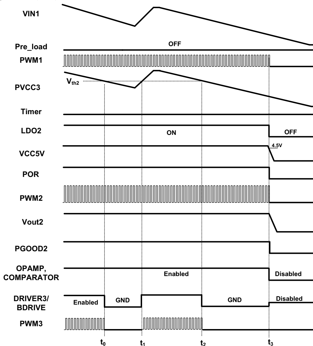
FIGURE 27. POWER-DOWN SEQUENCE
