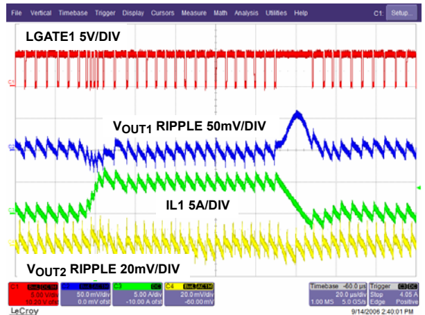
FIGURE 62. LOAD TRANSIENT V_{OUT1} = 1.5V (PWM)
